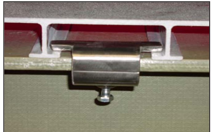
Unique Beam Clip Connection
