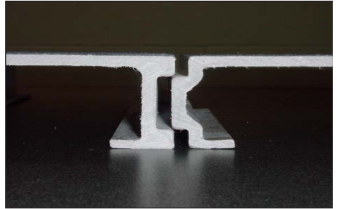
Tongue and Groove Connection
