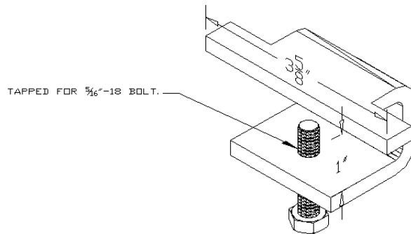
Heavy Duty Beam Clip Mount
